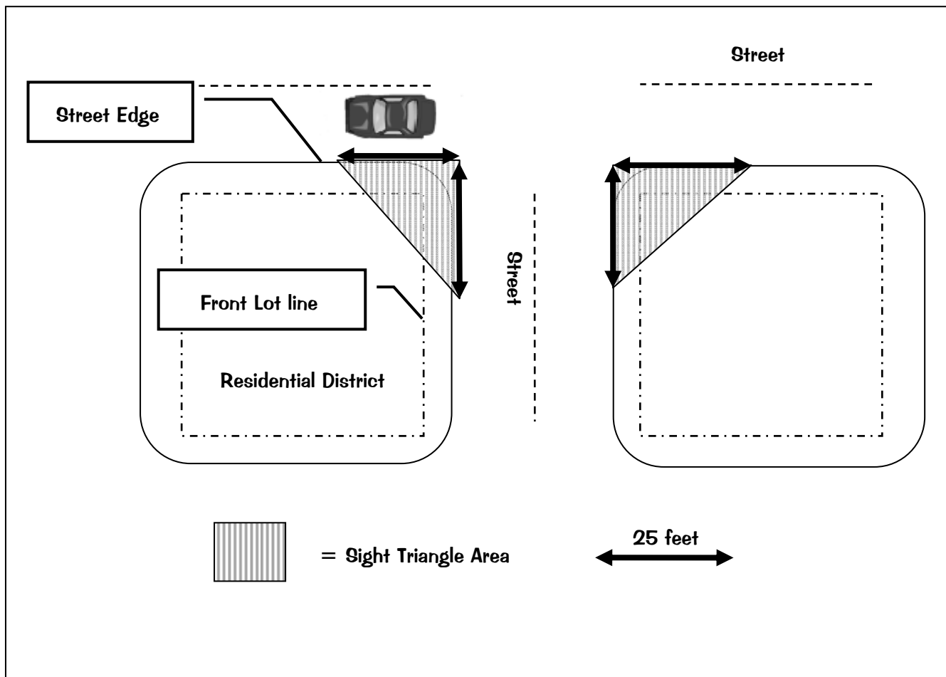
Figure 5-2 Sight Triangle
