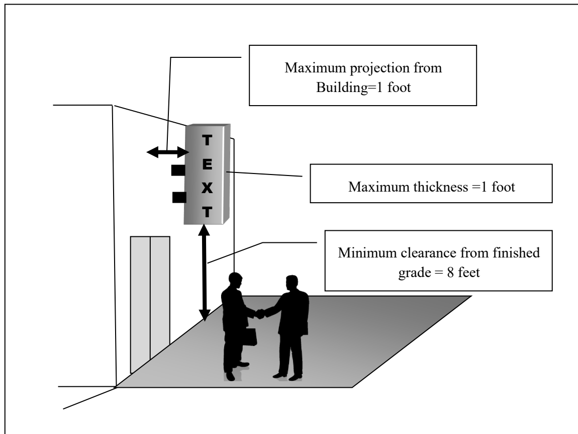
Figure 9-9 Projecting Sign
