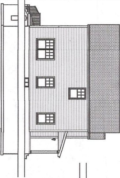
LEFT ELEVATION
