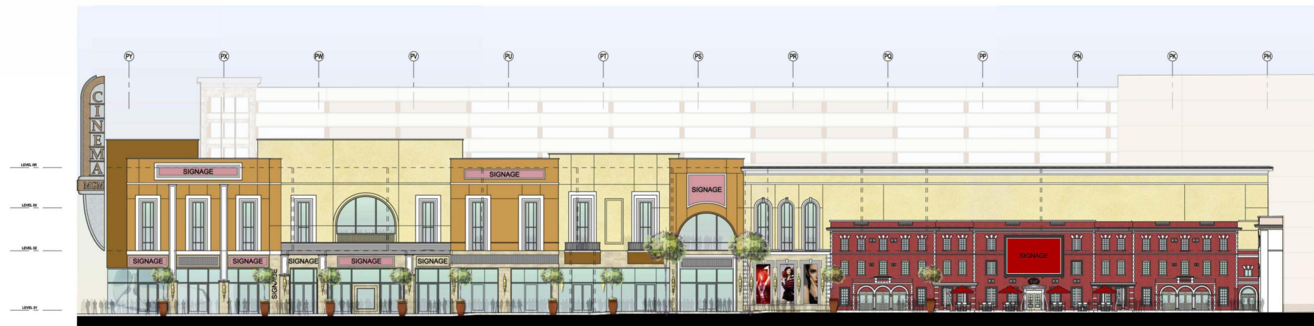
PLAZA ENTERTAINMENT ELEVATION
