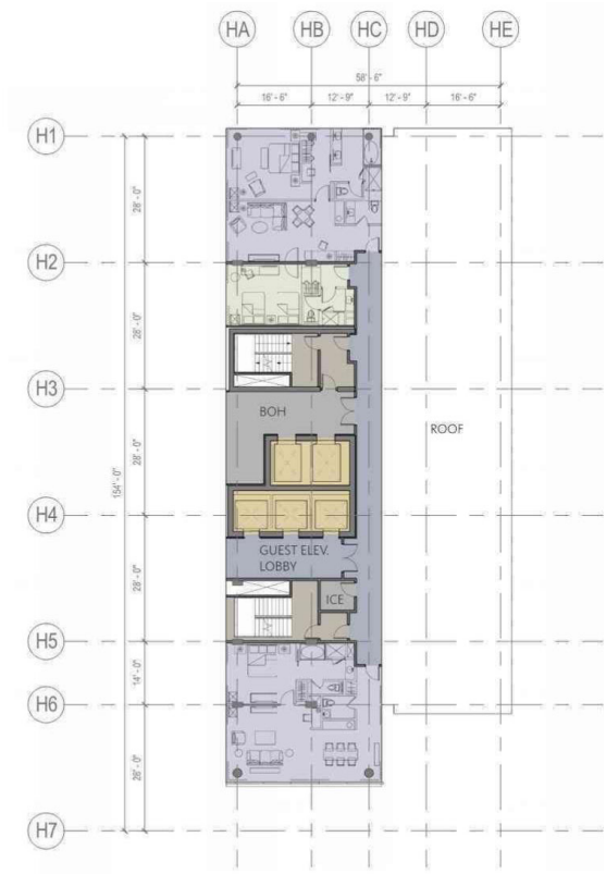
23 FLOOR OVERALL PLANS - LEVELS 22
