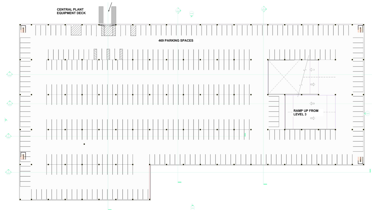
GARAGE LEVEL THREE
