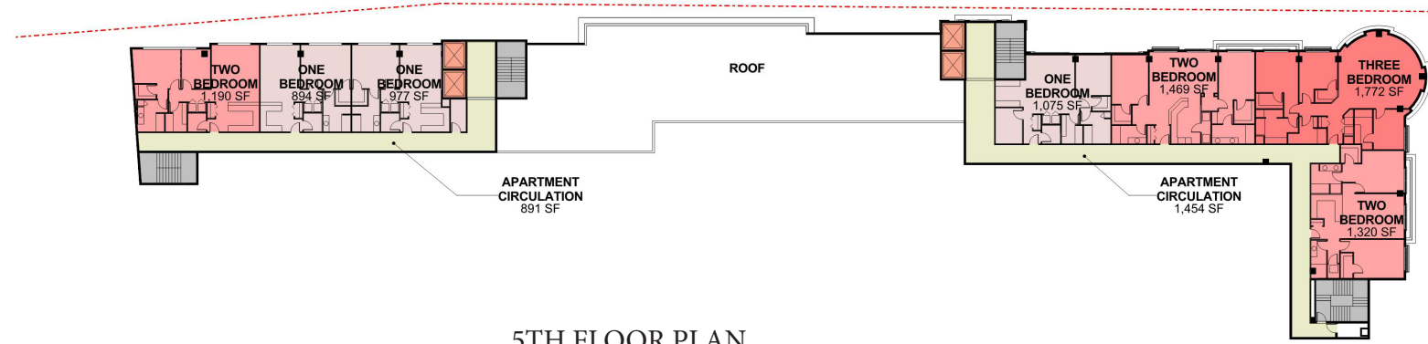
5TH FLOOR PLAN
