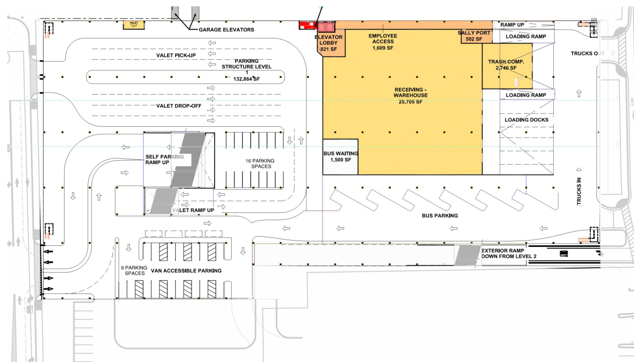
GARAGE LEVEL ONE
