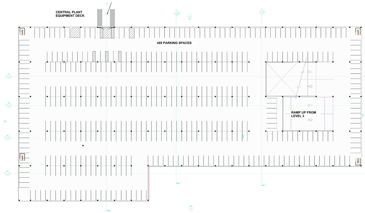
GARAGE LEVEL FOUR
